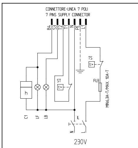
Fig. 25 - Conector 7-polos
